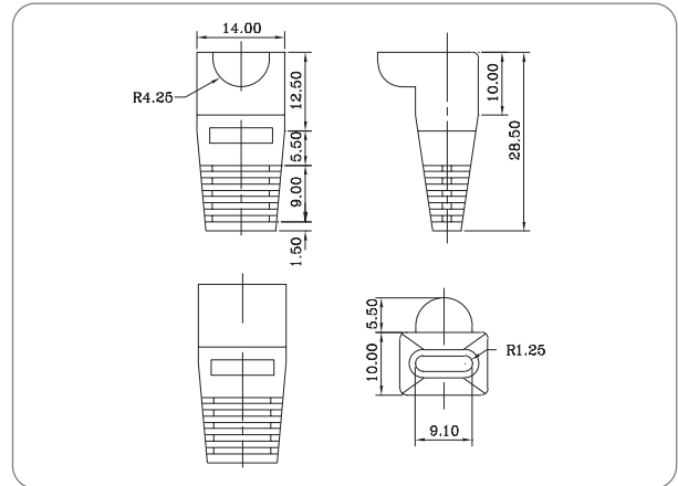
Cover for 8P Plug/Flat cable type
