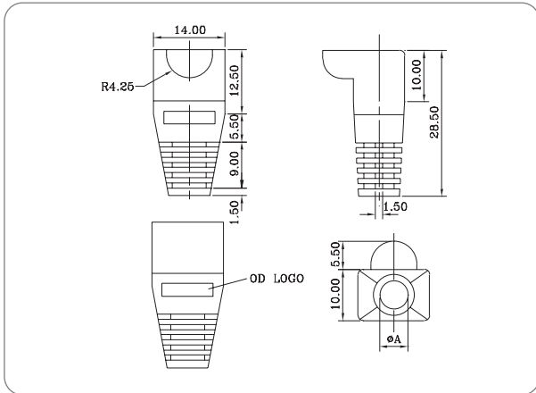
Cover for RJ45 Plug
