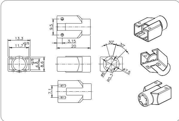
Design to fit Telebox 8P8C/10P10C fully shielded plugs TA5708FS/TA5710FS
