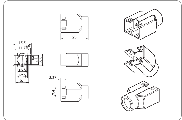
Design to fit Telebox 8P8C fully shielded plugs TA5708PC (Hirose type)
