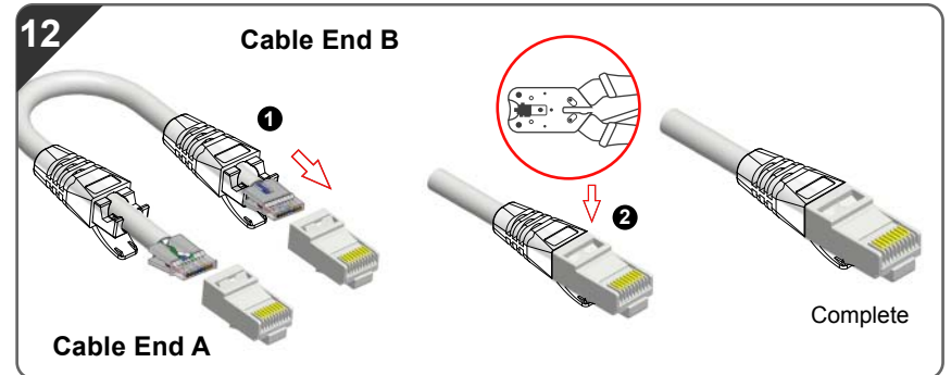
■ Note3: Wired-organizers has two directions for both ends. ■ Fasten boot into plug first then crimp and terminate the wires.
