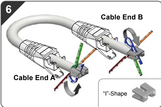
■ Insert blue-pair 4&5 to "I"-shape organizer tunnel. Note: 1. If blue-pair 4&5 be parallel, insert to organizer directly. 2. If blue-pair 4&5 be cross, twist with force insert parallel to organizer. 3. Organizer top-bottom direction is opposite in both ends.
